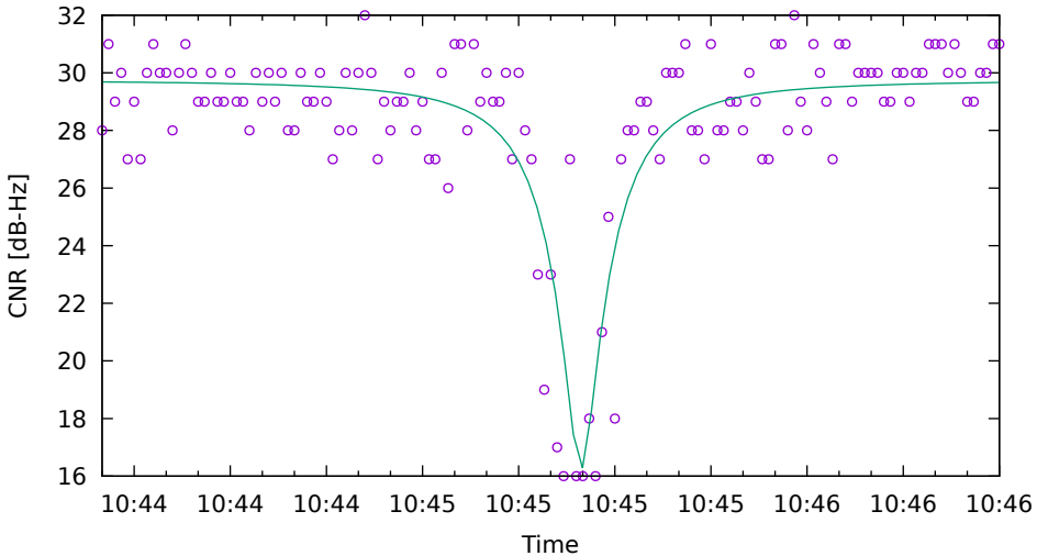
CNR fit for C26 on HuaweiP40 - drive 2 (DOY262)
