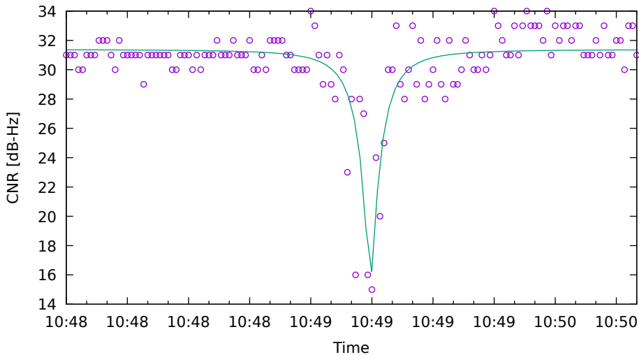
CNR fit for C26 on HuaweiP40 - drive 4 (DOY262)
