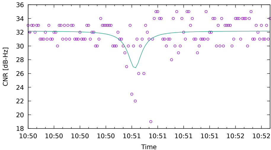
CNR fit for C26 on HuaweiP40 - drive 5 (DOY262)
