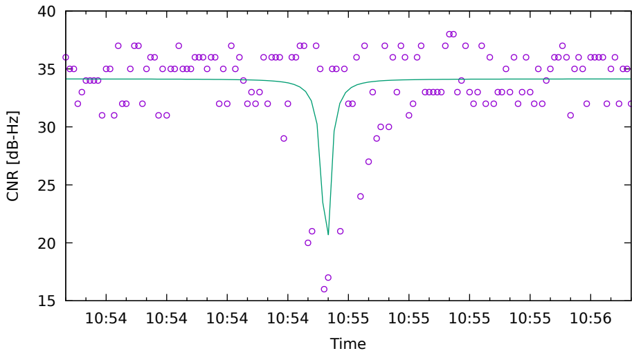
CNR fit for C26 on HuaweiP40 - drive 7 (DOY262)
