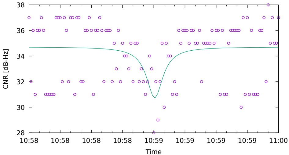
CNR fit for C26 on HuaweiP40 - drive 9 (DOY262)
