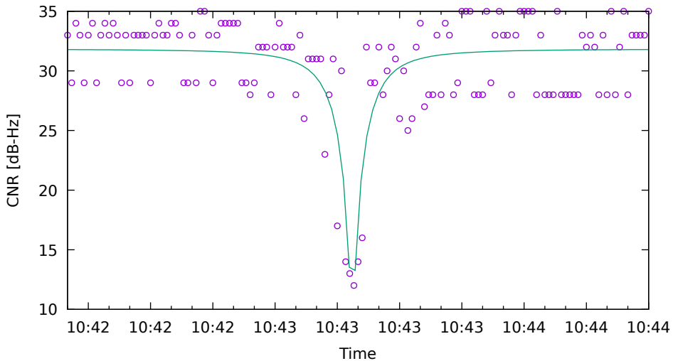
CNR fit for C27 on HuaweiP40 - drive 1 (DOY262)
