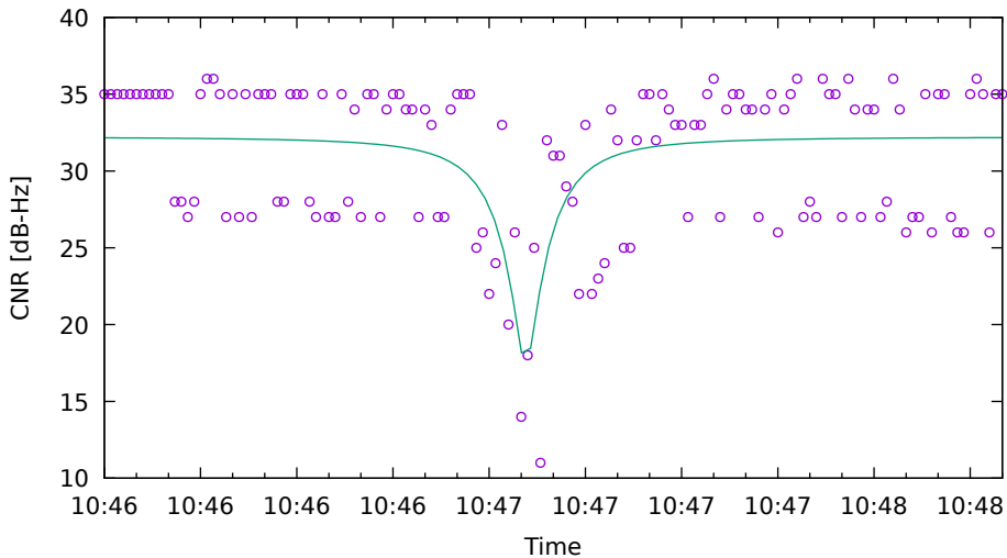
CNR fit for C27 on HuaweiP40 - drive 3 (DOY262)
