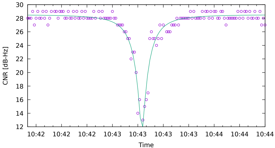
CNR fit for E05 on HuaweiP40 - drive 1 (DOY262)
