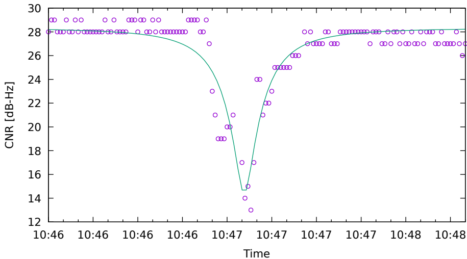
CNR fit for E05 on HuaweiP40 - drive 3 (DOY262)
