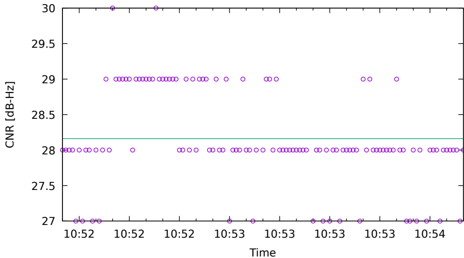
CNR fit for E05 on HuaweiP40 - drive 6 (DOY262)
