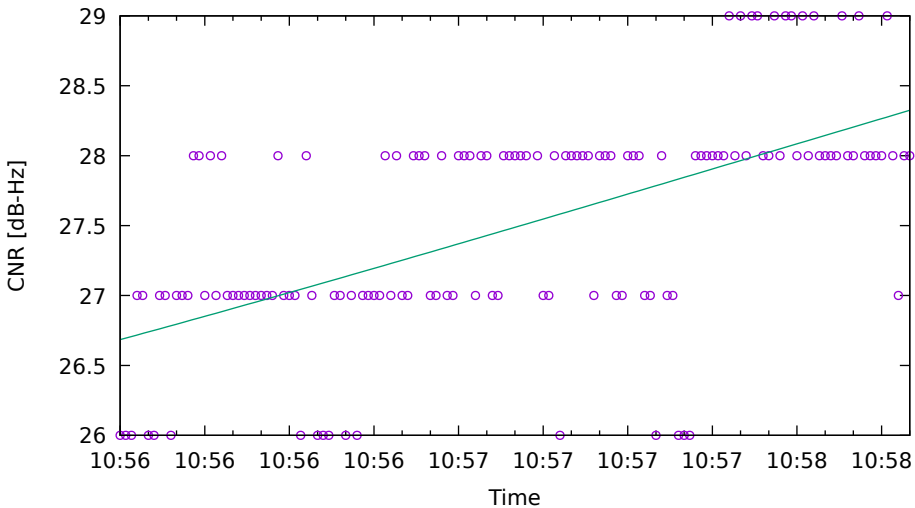
CNR fit for E05 on HuaweiP40 - drive 8 (DOY262)
