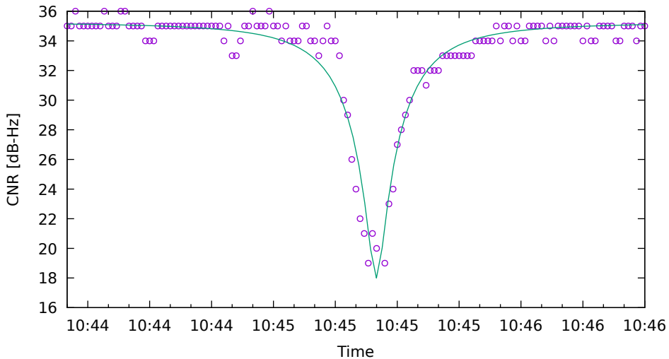
CNR fit for E09 on HuaweiP40 - drive 2 (DOY262)
