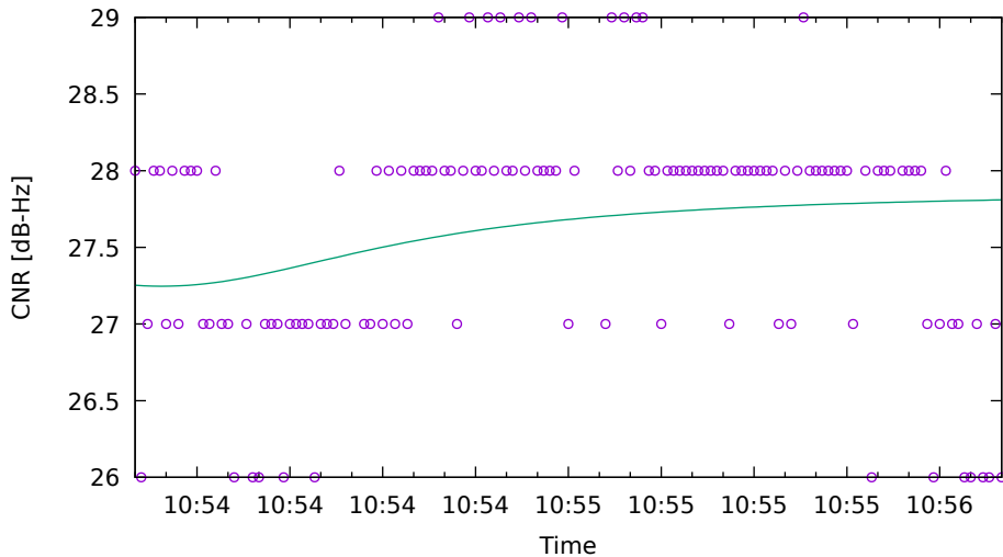
CNR fit for E09 on HuaweiP40 - drive 7 (DOY262)
