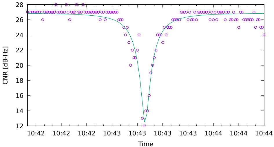
CNR fit for E36 on HuaweiP40 - drive 1 (DOY262)
