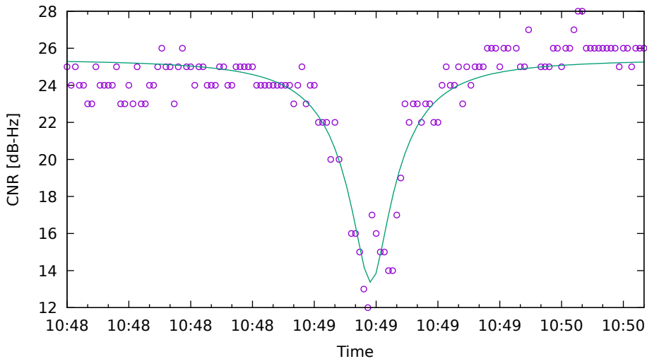
CNR fit for E36 on HuaweiP40 - drive 4 (DOY262)
