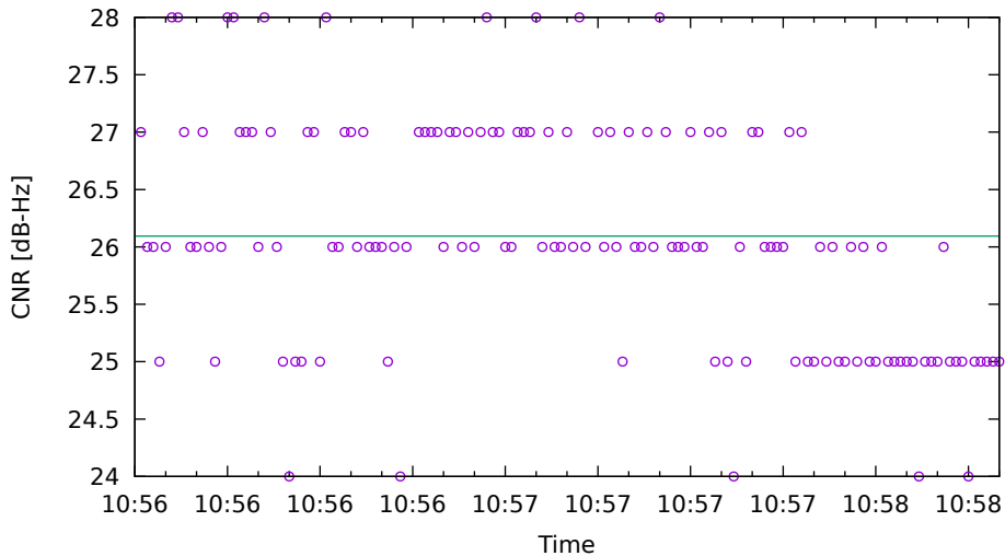
CNR fit for E36 on HuaweiP40 - drive 8 (DOY262)
