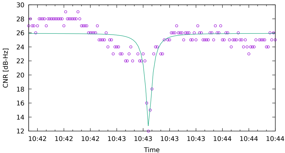
CNR fit for G01 on HuaweiP40 - drive 1 (DOY262)
