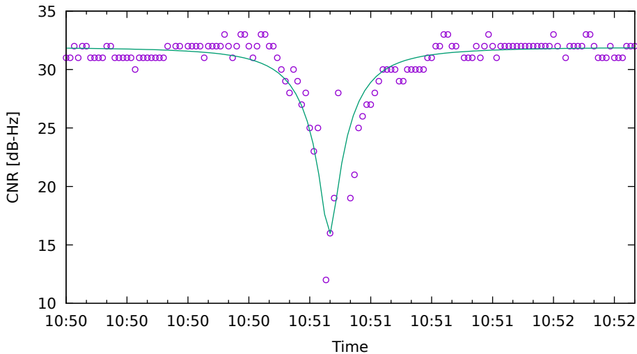
CNR fit for G01 on HuaweiP40 - drive 5 (DOY262)
