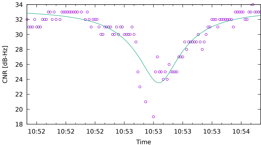
CNR fit for G01 on HuaweiP40 - drive 6 (DOY262)
