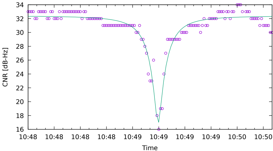
CNR fit for G03 on HuaweiP40 - drive 4 (DOY262)
