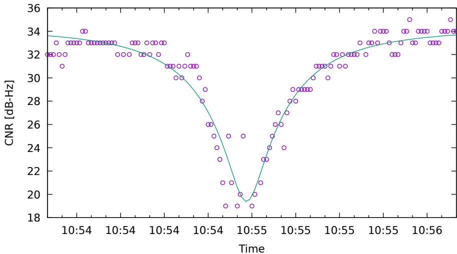
CNR fit for G03 on HuaweiP40 - drive 7 (DOY262)
