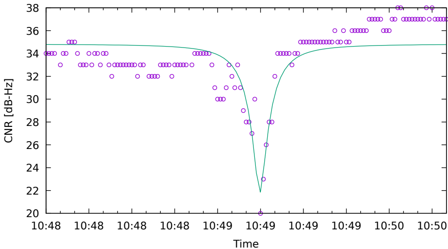
CNR fit for G09 on HuaweiP40 - drive 4 (DOY262)
