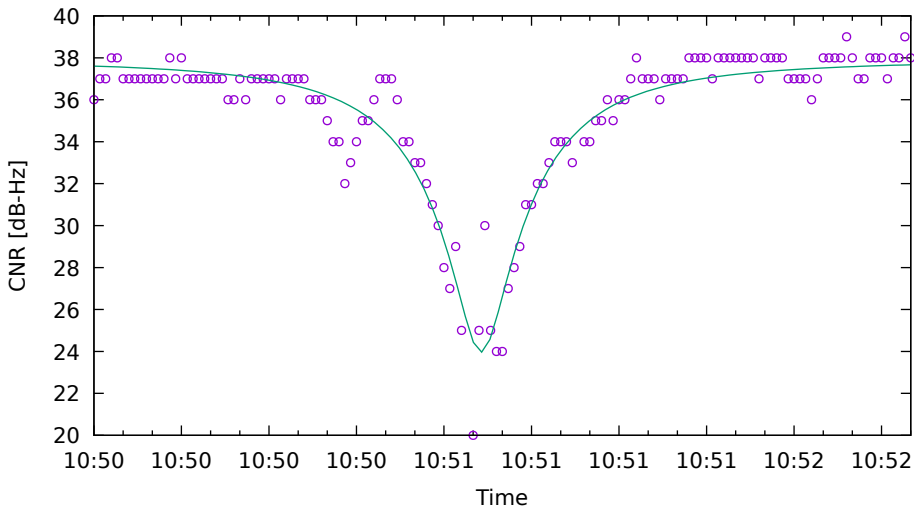
CNR fit for G09 on HuaweiP40 - drive 5 (DOY262)
