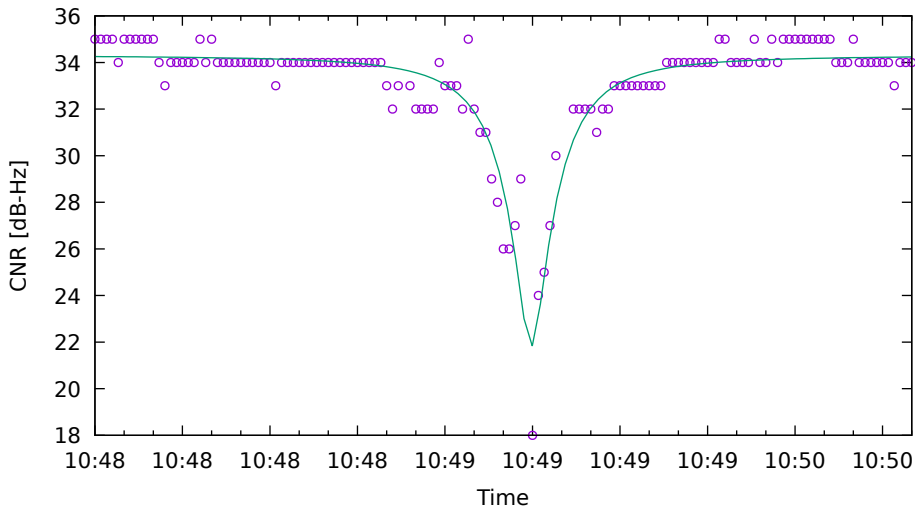
CNR fit for G19 on HuaweiP40 - drive 4 (DOY262)
