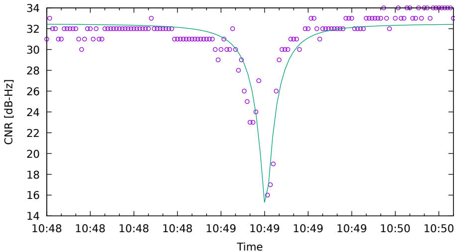
CNR fit for G21 on HuaweiP40 - drive 4 (DOY262)
