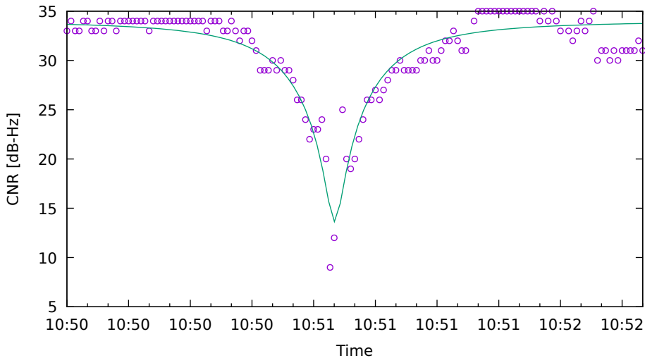
CNR fit for G21 on HuaweiP40 - drive 5 (DOY262)
