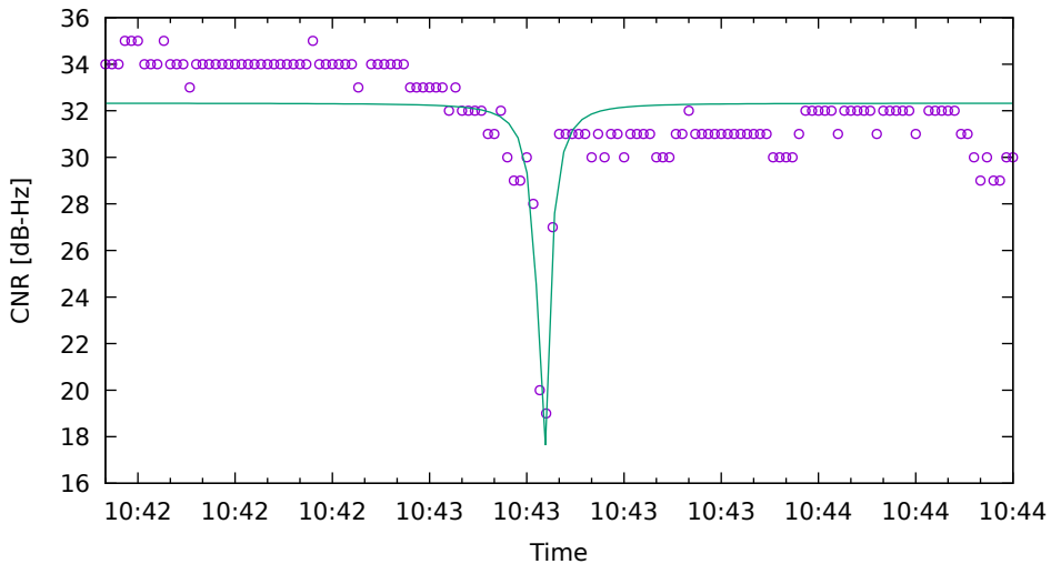
CNR fit for G22 on HuaweiP40 - drive 1 (DOY262)
