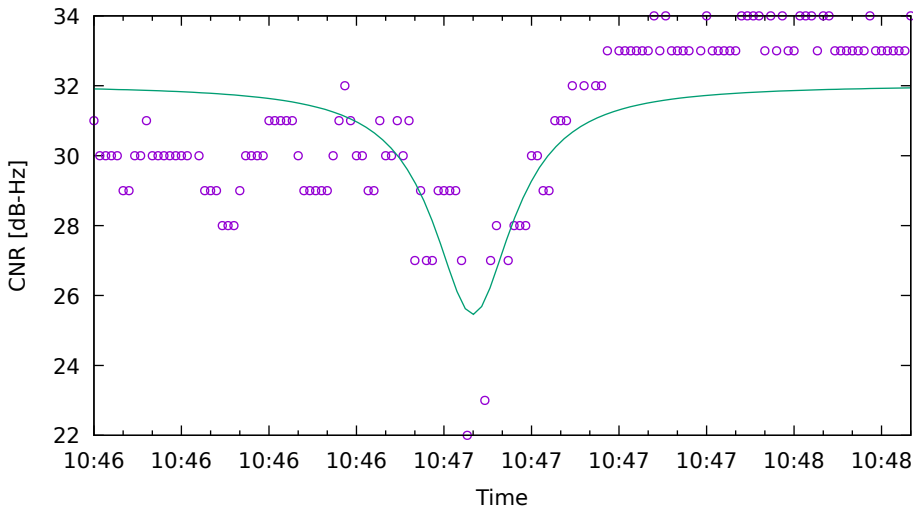
CNR fit for G22 on HuaweiP40 - drive 3 (DOY262)
