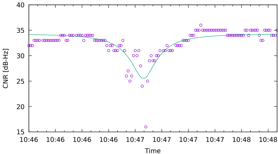
CNR fit for G31 on HuaweiP40 - drive 3 (DOY262)
