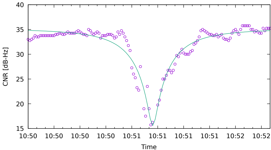
CNR fit for E05 on XiaomiMi8 - drive 5 (DOY262)
