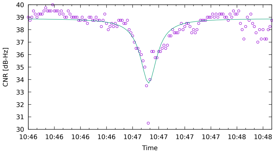
CNR fit for E09 on XiaomiMi8 - drive 3 (DOY262)
