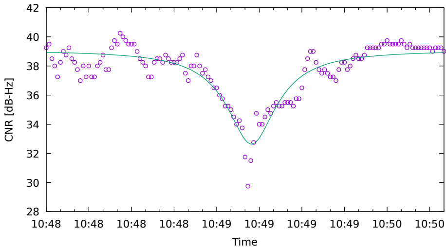
CNR fit for E09 on XiaomiMi8 - drive 4 (DOY262)
