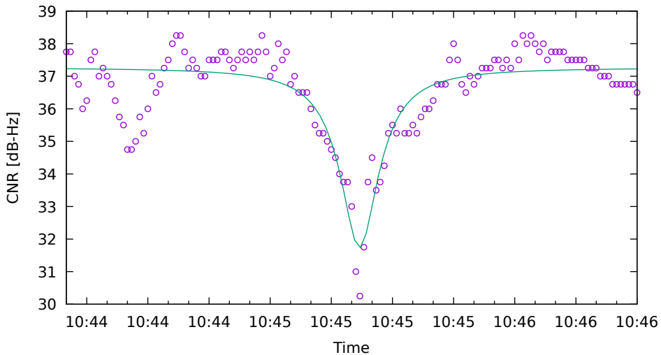
CNR fit for E36 on XiaomiMi8 - drive 2 (DOY262)
