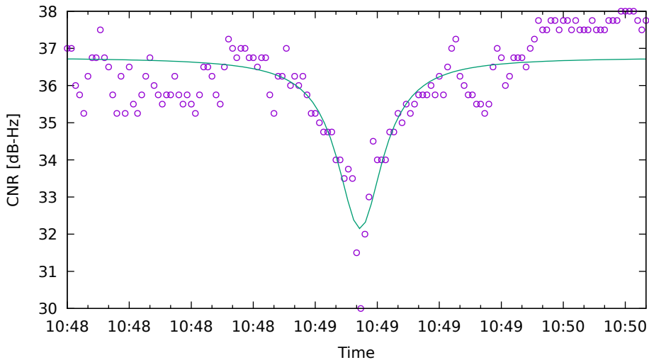
CNR fit for E36 on XiaomiMi8 - drive 4 (DOY262)
