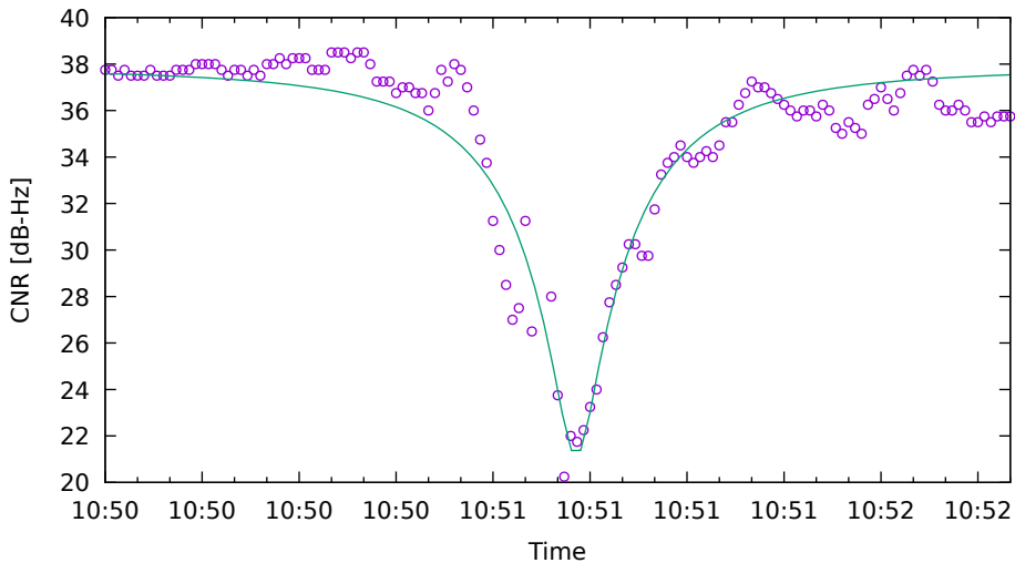
CNR fit for E36 on XiaomiMi8 - drive 5 (DOY262)
