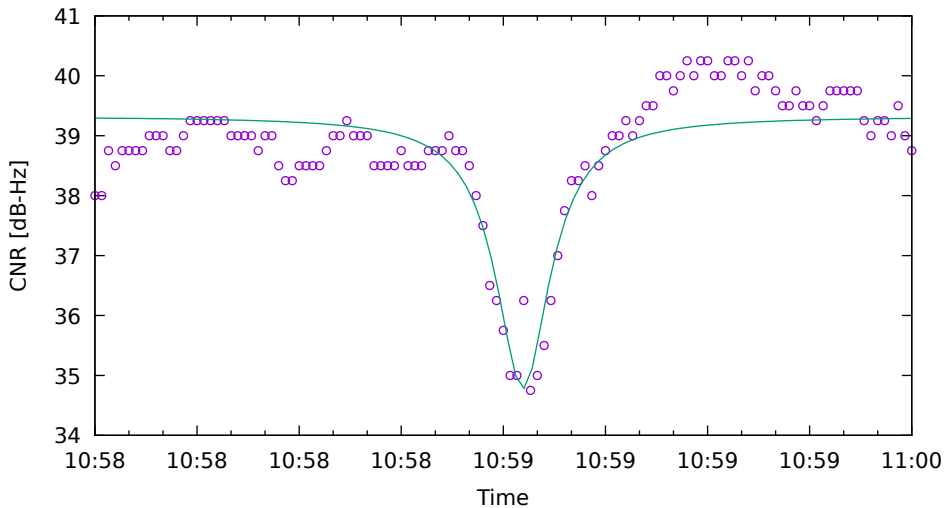
CNR fit for E36 on XiaomiMi8 - drive 9 (DOY262)
