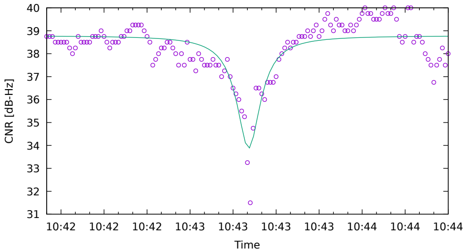
CNR fit for G03 on XiaomiMi8 - drive 1 (DOY262)
