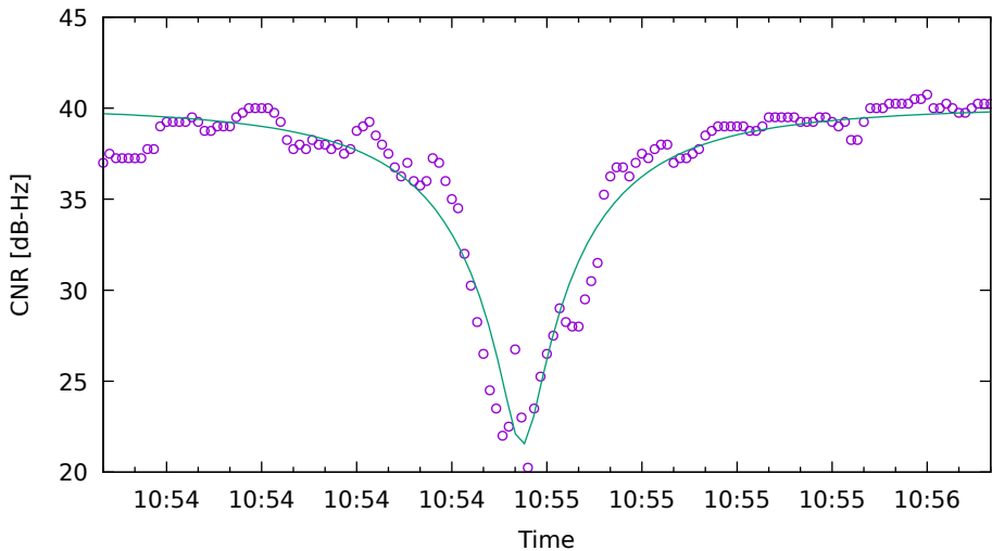
CNR fit for G03 on XiaomiMi8 - drive 7 (DOY262)
