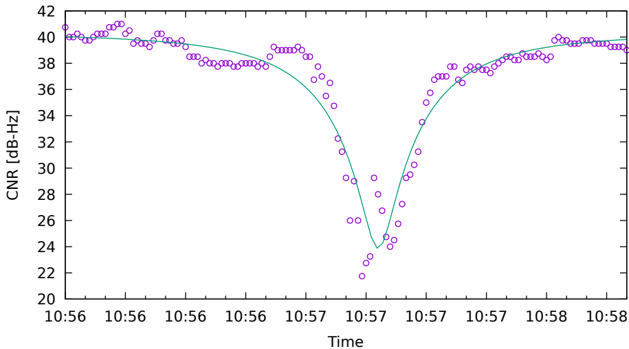
CNR fit for G03 on XiaomiMi8 - drive 8 (DOY262)
