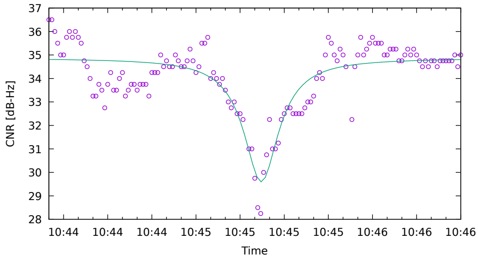
CNR fit for G04 on XiaomiMi8 - drive 2 (DOY262)
