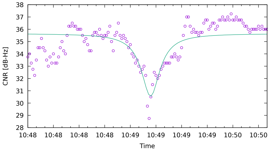
CNR fit for G04 on XiaomiMi8 - drive 4 (DOY262)
