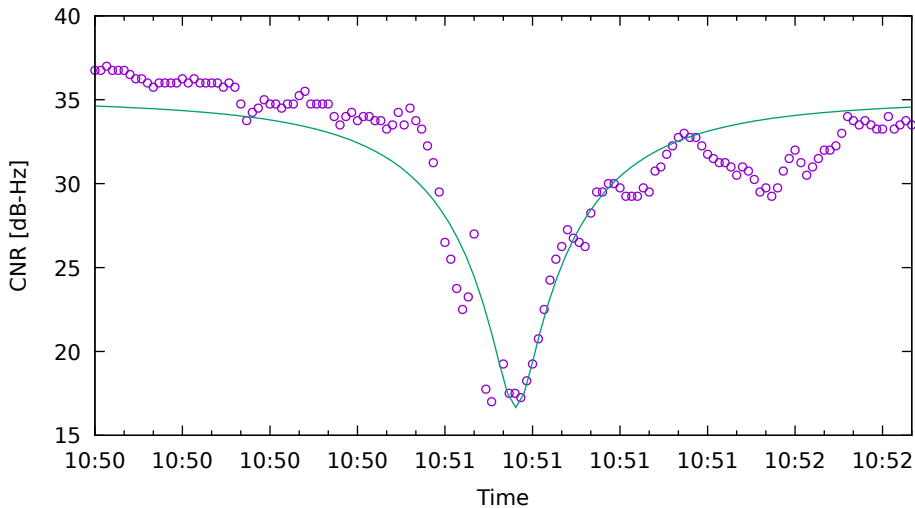
CNR fit for G04 on XiaomiMi8 - drive 5 (DOY262)
