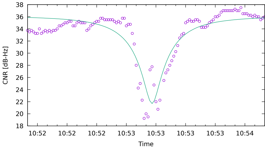
CNR fit for G04 on XiaomiMi8 - drive 6 (DOY262)
