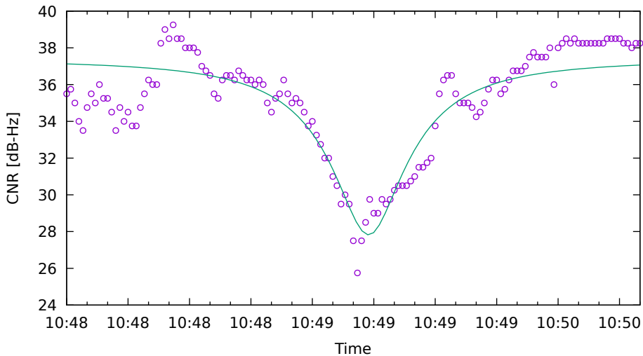
CNR fit for G19 on XiaomiMi8 - drive 4 (DOY262)
