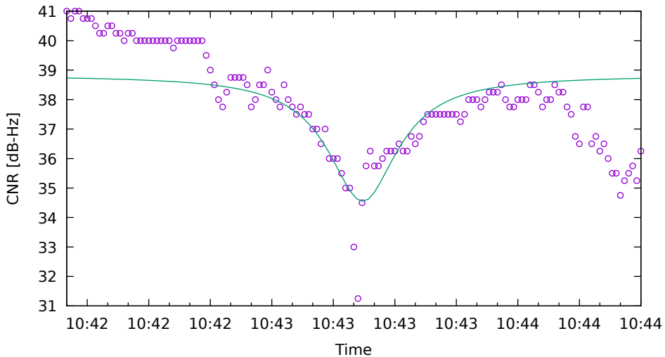
CNR fit for G21 on XiaomiMi8 - drive 1 (DOY262)
