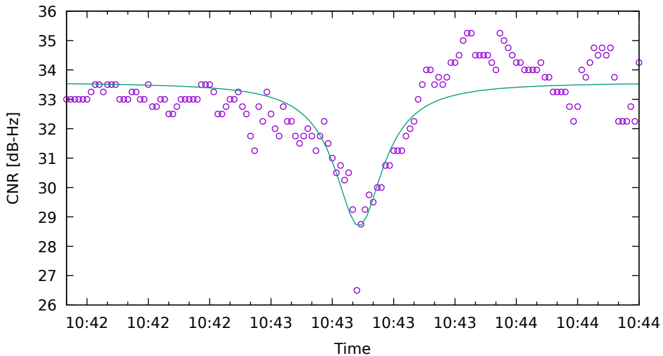
CNR fit for G22 on XiaomiMi8 - drive 1 (DOY262)
