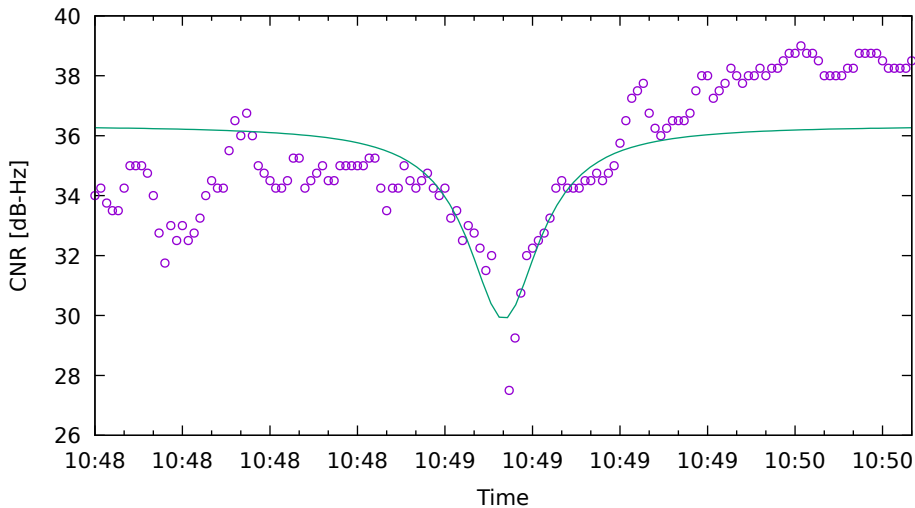
CNR fit for G22 on XiaomiMi8 - drive 4 (DOY262)
