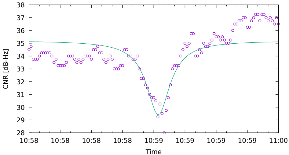
CNR fit for G22 on XiaomiMi8 - drive 9 (DOY262)
