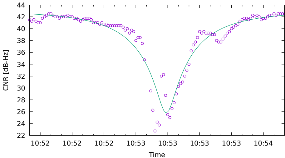
CNR fit for G31 on XiaomiMi8 - drive 6 (DOY262)
