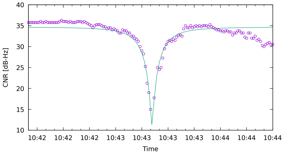
CNR fit for R01 on XiaomiMi8 - drive 1 (DOY262)
